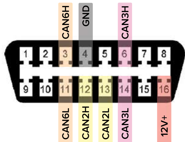
Front view of OBD interface
