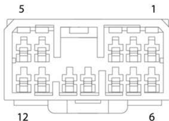
Front View of Male Car Interface
